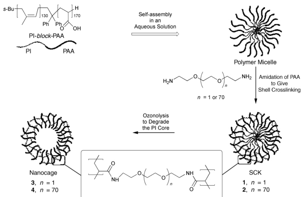
Fig. 5 Procedure for the preparation of nanocapsules from amphiphilic diblock copolymers. The shell of the final nanocapsules consists of crosslinked poly(acrylamide). (Reproduced with permission from J. Am. Chem. Soc. , 1999, 121 , 3805.)
