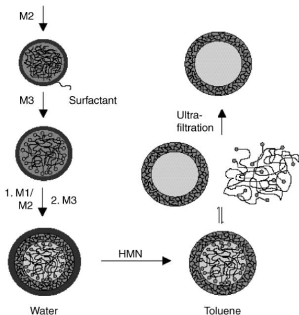
Fig. 8 Preparation of organosilicon nanocapsules. M1: \text{MeSi}(\text{OMe})_3 , M2: \text{Me}_2\text{Si}(\text{OMe})_2 , M3: \text{Me}_3\text{SiOMe} , HMN: hexamethyldisilazane. (Reproduced with permission from Adv. Mater. , 1999, 11 , 1299.)
